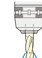
A front nut with an O-ring seal, for use with oil hole cutter, is also available as option.
