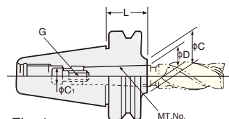
Draw bolt type
