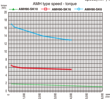
ANGULAR HEAD(AHM) speed(min -1 )-torque(Nm)/power(kW)
